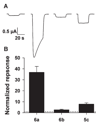
Figure 3. Direct quantitative comparison of steroids 6a, 6b, and 5c at 10 \mu M on responses to GABA in Xenopus oocytes expressing \alpha_1\beta_2\gamma_{2L} GABA A receptor subunits. (A) Responses to 2 \mu M GABA alone (left trace) and to GABA coapplied with 10 \mu M each of 6a (second trace), 6b (third trace), and 5c (right trace). All responses are from the same oocyte. (B) Summary of responses in which 6a, 6b, and 5c were tested within oocytes, normalized to the response of GABA alone in each oocyte. The normalizing response is indicated with a dotted horizontal line at y = 1 ( N = 4 ). Error bars are SEM.
