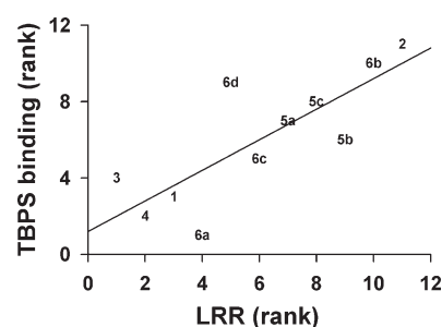
Figure 5. Rank order correlation plot of the analogue [ 35 S]TBPS IC 50 with their corresponding tadpole LRR EC 50 . Compound numbers are used to represent data points on the plot. The correlation is significant; r = 0.8 ( p < 0.05 ).
