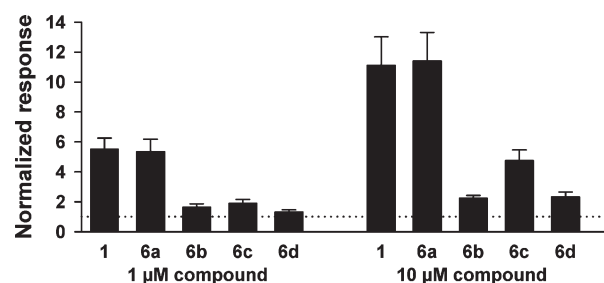
Figure 4. Summary of normalized responses of oocytes to coapplied GABA (2 \mu M) plus 1 \mu M (left set of bars) or 10 \mu M (right set of bars) of the indicated compounds, tested within oocytes. The normalizing response of GABA alone is indicated by the horizontal dotted line at y = 1 . Bars represent mean responses of six to seven oocytes for each compound. Error bars are SEM.
